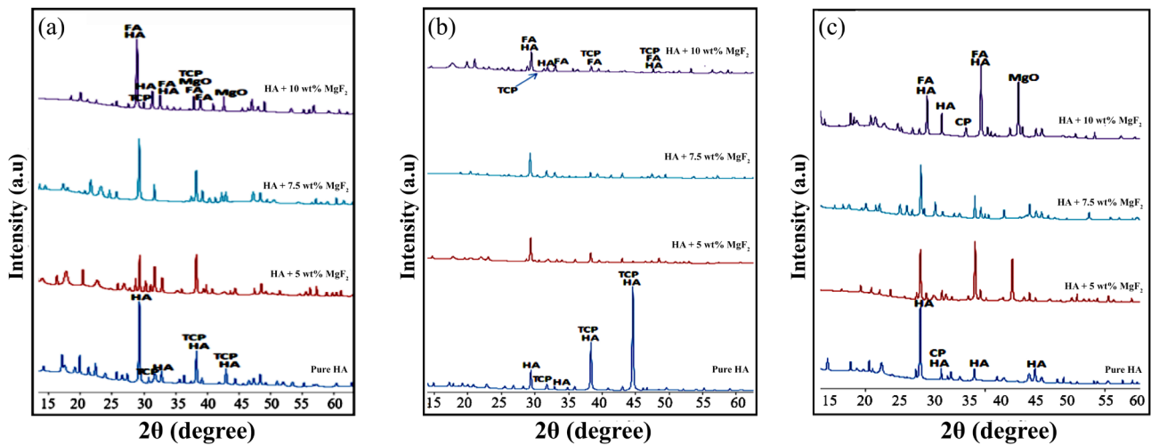
Fig. 2. X-ray diffraction spectra for specimens containing different percentages of \text{MgF}_2 sintered for 1 hour at (a) 900 °C, (b) 1000 °C, and (c) 1100 °C.
