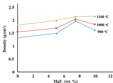
Fig. 3. Density variations of the specimens as percentage of \text{MgF}_2 at different temperatures of sintering.
