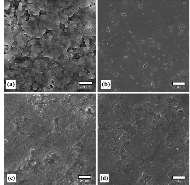
Fig. 6. SEM images of sintered specimens at 1100 °C: (a) 0 wt.% MgF 2 ; b) 5 wt.% MgF 2 ; c) 7.5 wt.% MgF 2 ; d) 10 wt.% MgF 2 .
