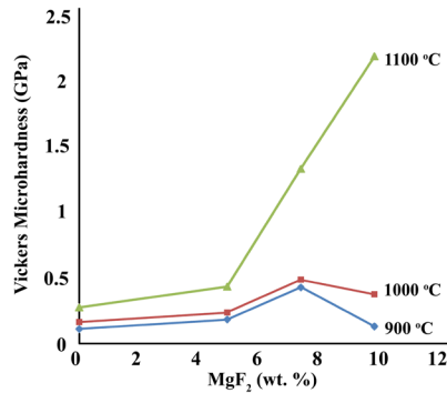
Fig. 7. Micro hardness values by weight percent of MgF 2 at different temperatures.
