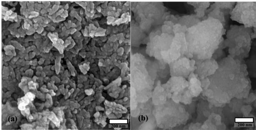
Fig. 1. SEM image of (a) HA powder and (b) primary \text{MgF}_2 powder.
